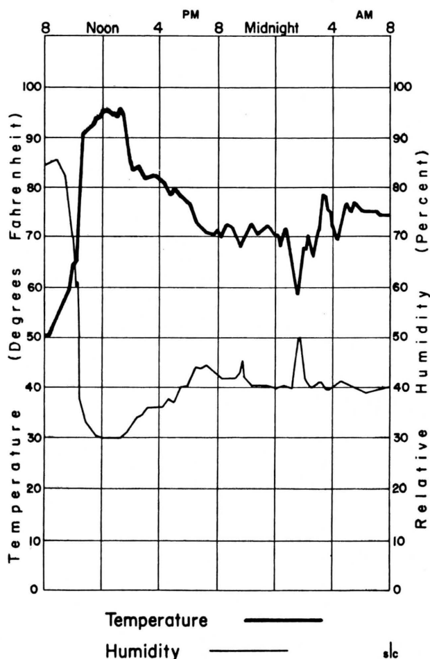
Fig. 6. Atypical temperature and humidity pattern at Swakopmund.
