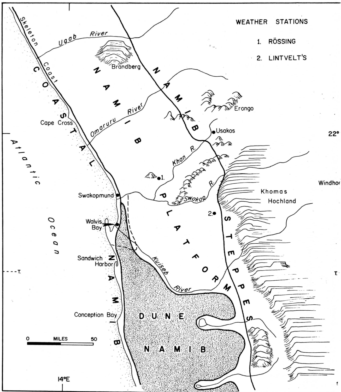
Fig. 2. Regional divisions of the central Namib Desert.
